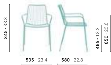
3656 Steel armchair, high backrest
