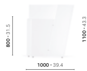
OBA_BI corner Corner module in polyethylene
